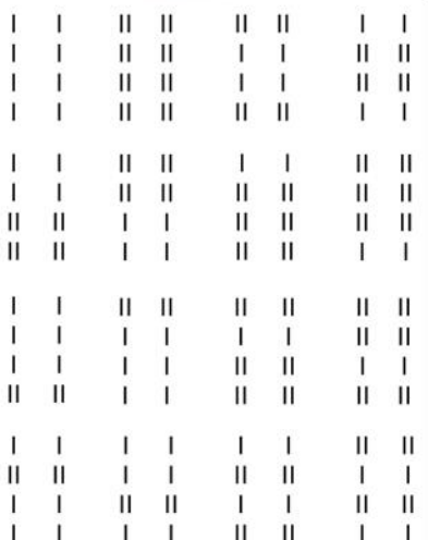
Opon Ifa Binary System (64 Combinations)
