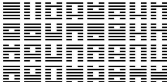
I-Ching Binary System (64 Hexagrams)
